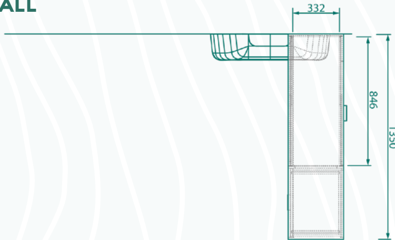
REAR INSTALL - PLAN VIEW
