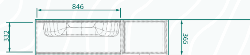
SIDE INSTALL - PLAN VIEW
