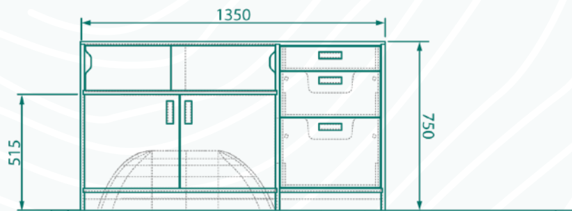
SIDE INSTALL - FRONT VIEW
